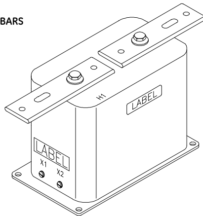
Model CTWH5-L WITH PRIMARY BARS
