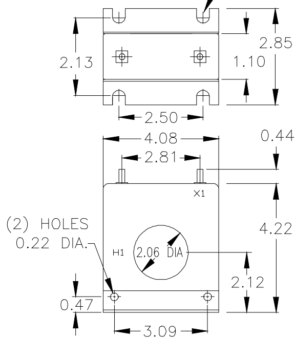
Model 6ASHT (4) OPEN SLOTS 0.22 X 0.47
