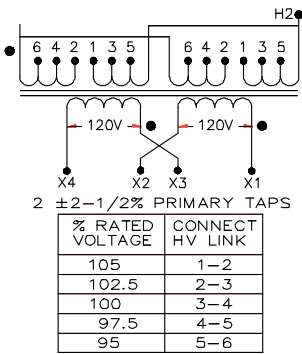
CONNECTION DIAGRAM "B"
