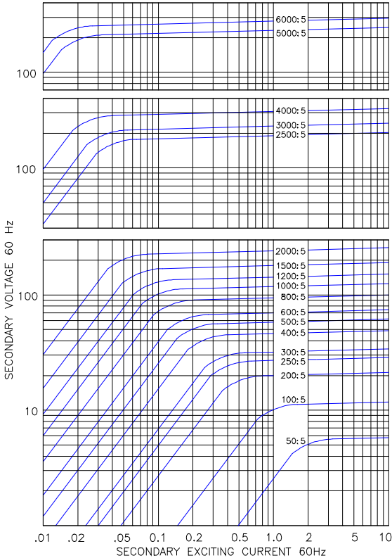
EXCITATION CURVE
