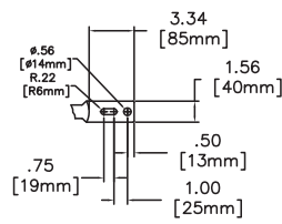
Primary Terminal
