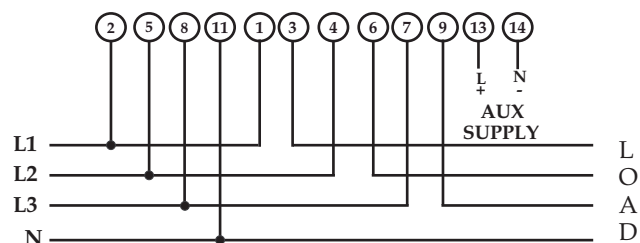
For 3 Phase 3 Wire Unbalanced Load
