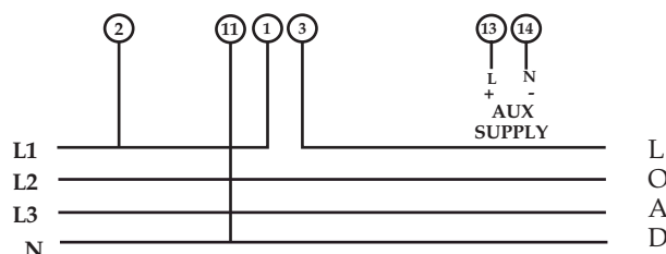
For Single Phase
