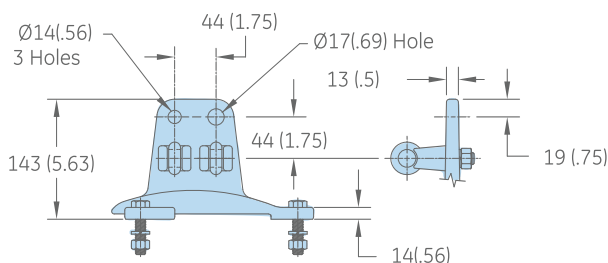
4 Hole NEMA Terminal
