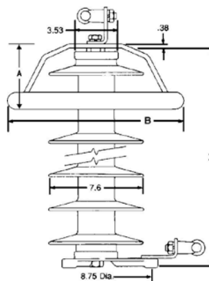
Eyebolt Terminal — Drawing 2A
