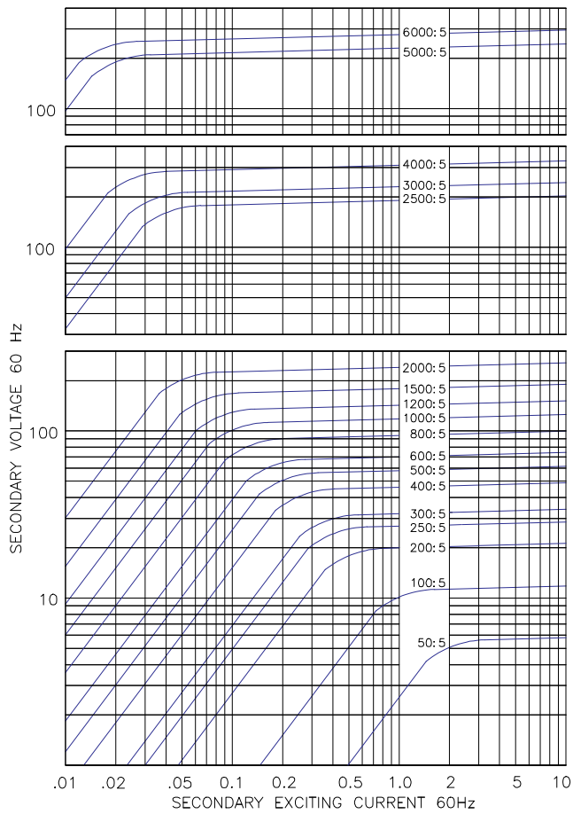
EXCITATION CURVE
