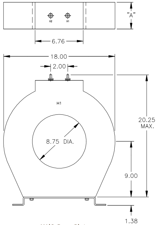
W/O Base Plate View
