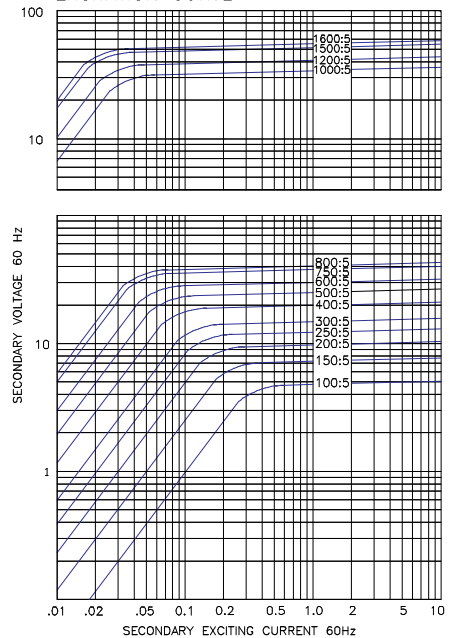
EXCITATION CURVE
