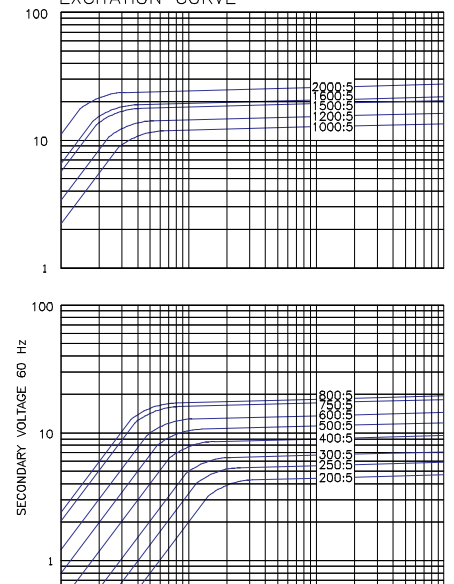
EXCITATION CURVE
