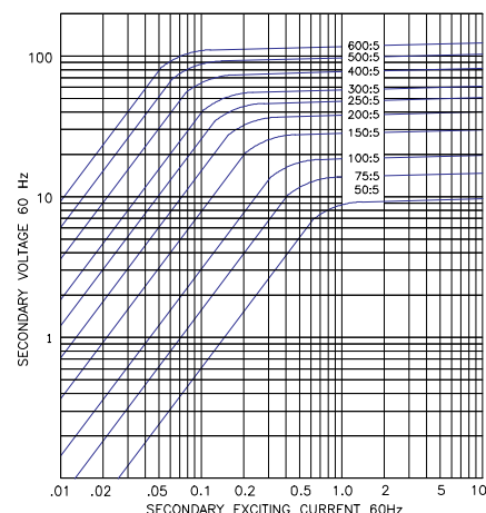
EXCITATION CURVE
