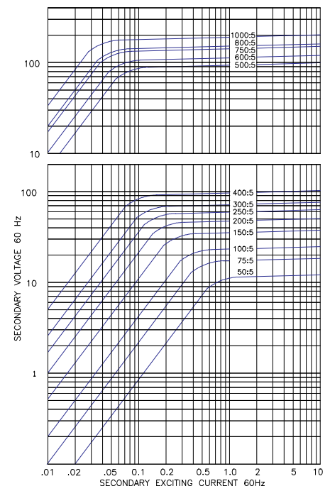
EXCITATION CURVE
