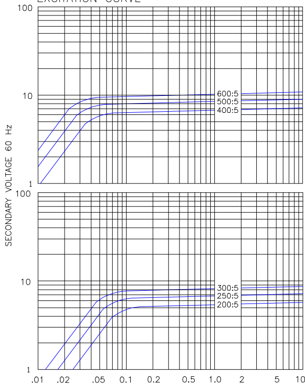
EXCITATION CURVE
