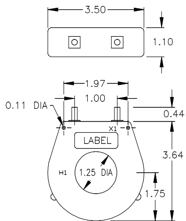
Model 58RT
