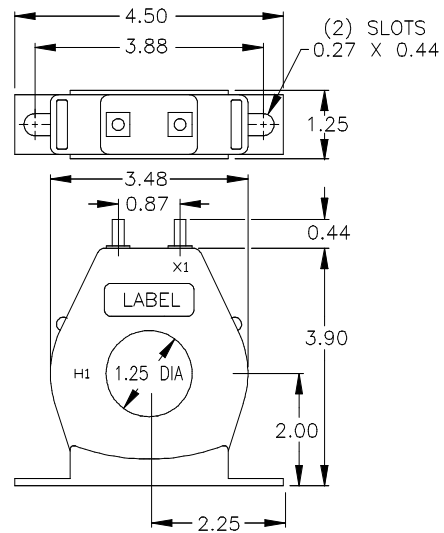
Model 58RBL
