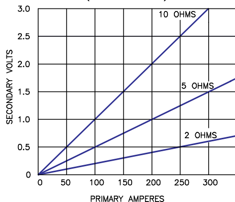
TYPICAL PERFORMANCE CHARACTERISTICS (WITH 1000 TURNS)
