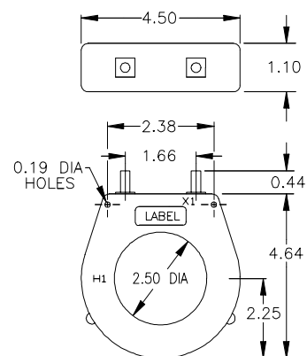
Model 7RT
