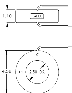
Model 7RL
