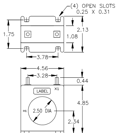
Model 7SFT
