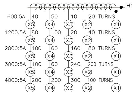
CONNECTION DIAGRAM
