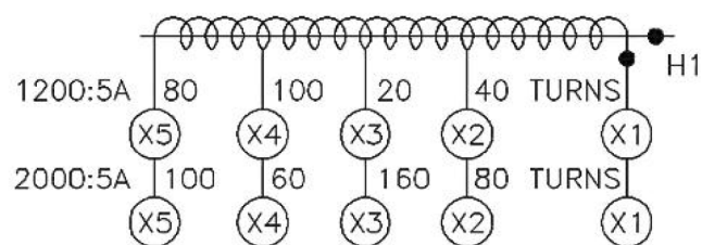
CONNECTION DIAGRAM
