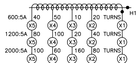
CONNECTION DIAGRAM
