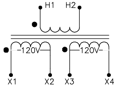
CONNECTION DIAGRAM
