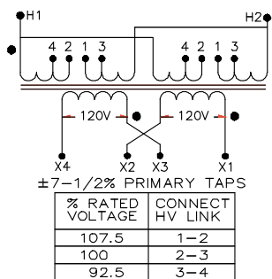
CONNECTION DIAGRAM "A"
