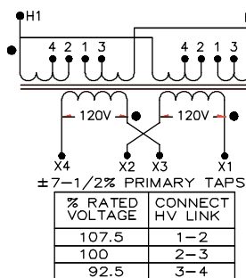
CONNECTION DIAGRAM "A"
