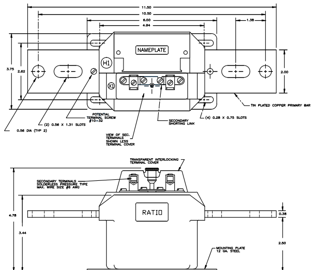
Current Ratio > 400:5
