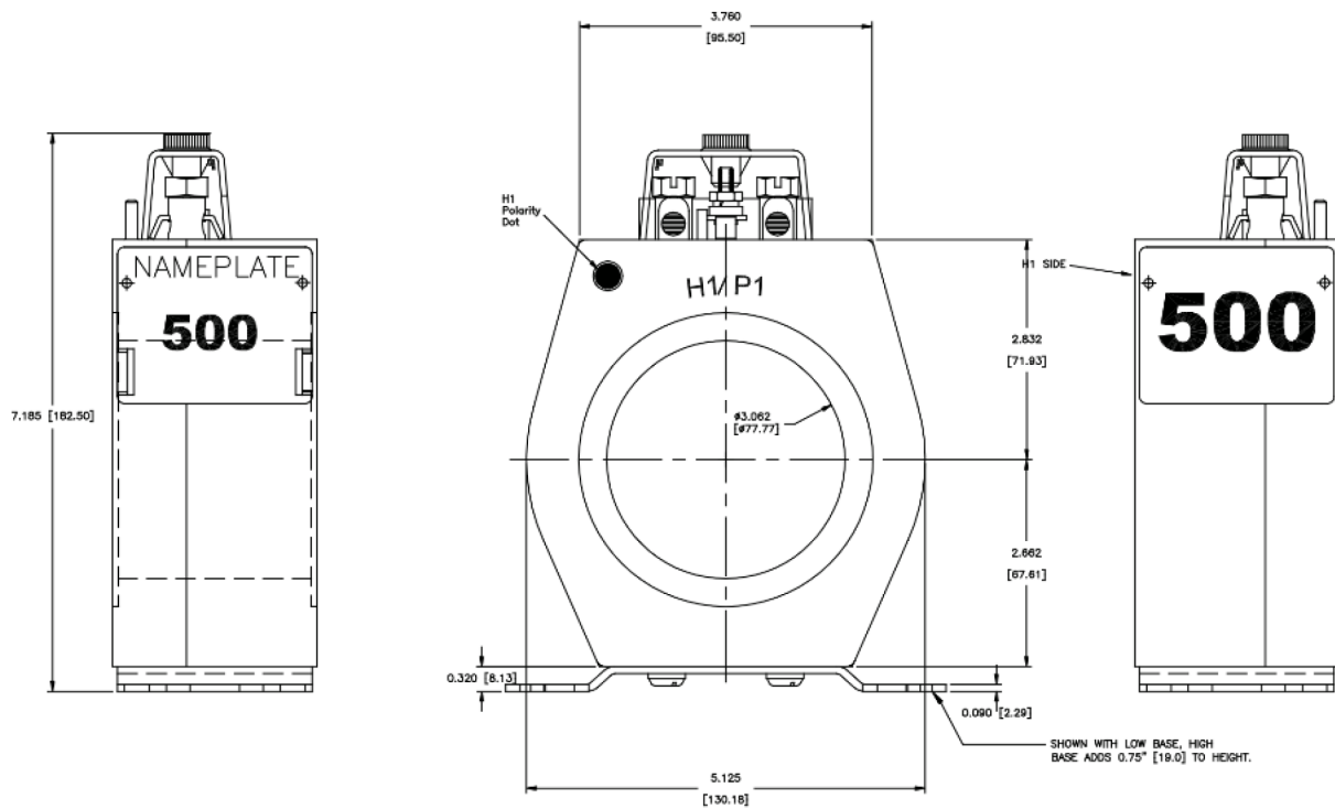
Outline drawings of JAK-OC model
