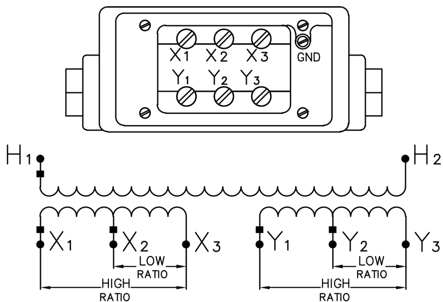
Dual-tapped secondary (Six secondary terminals)
