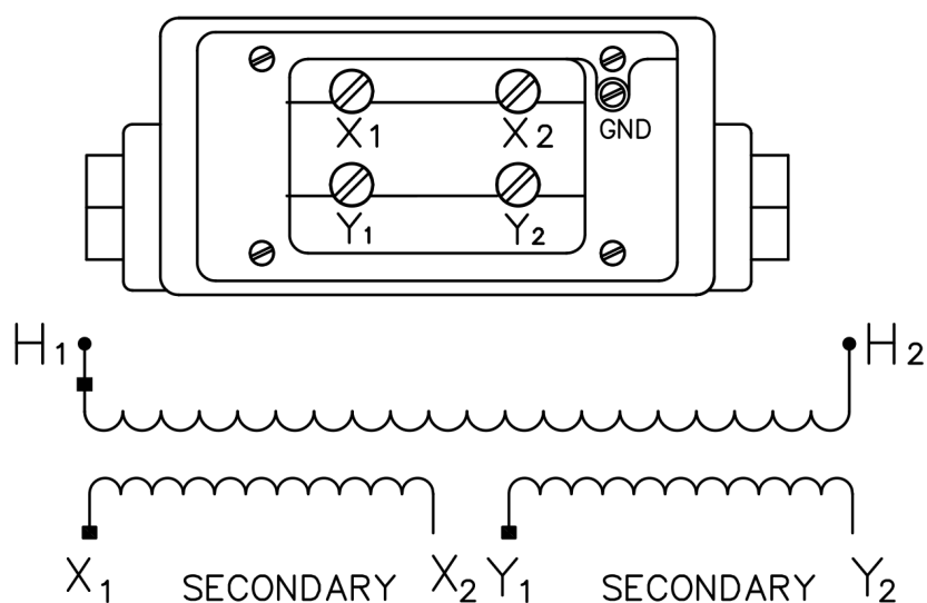
Dual Secondary (default) (Four secondary terminals)
