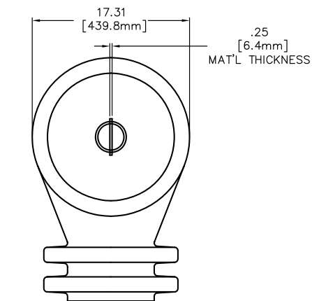
PAD CONFIGURATION FOR 800:5-1200:5 1 PAD EACH SIDE
