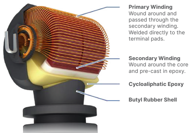
Cross-section View of a Station-Class SUPERBUTE Current Transformer
