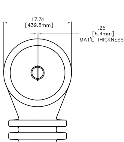
PAD CONFIGURATION FOR 800:5-1200:5 1 PAD EACH SIDE
