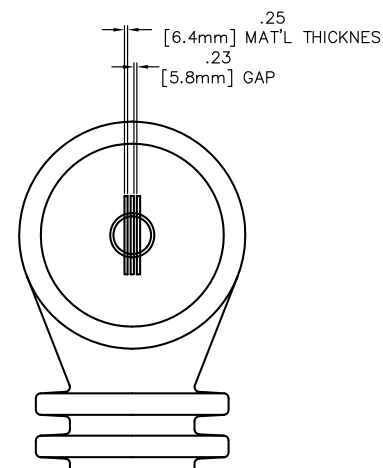
PAD CONFIGURATION FOR 3000:5 3 PADS EACH SIDE
