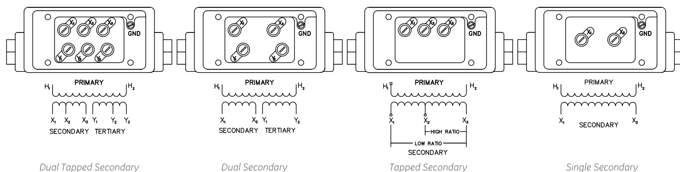
Dual Tapped Secondary
