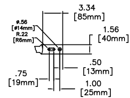
Primary Terminal
