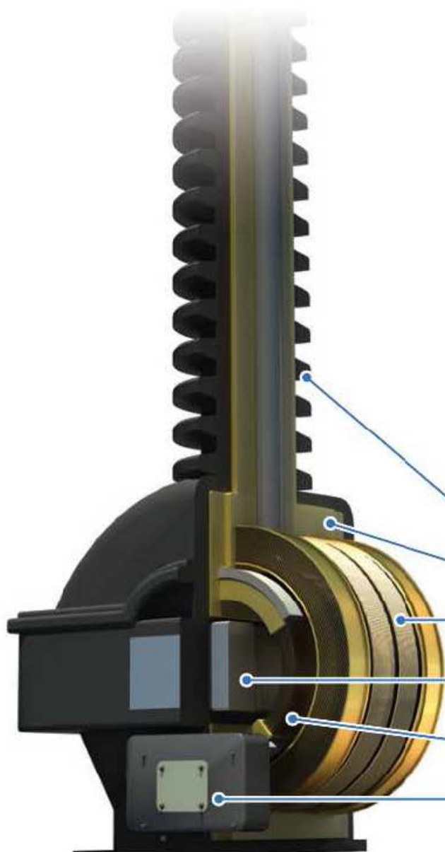
Cross-Section view of a Station-Class SUPERBUTE Vo/toge Transformer
