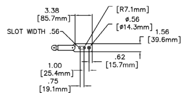
Primary Terminal
