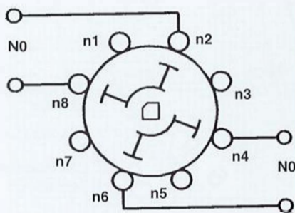
Figure 11 - Contact Deck Layout in both "RESET" and "TRIP" positions
