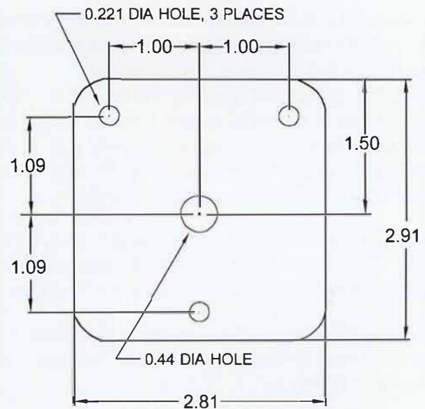
Figure 2 - Nameplate and Panel Drilling Dimensions
