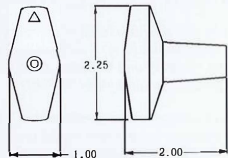
Figure 3 - Handle Dimensions
