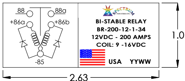
PRODUCT LABEL
